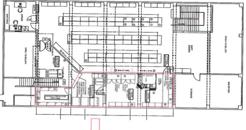
3 NEW LAYOUT-SECOND FLOOR 1/4" = 1'-0"
