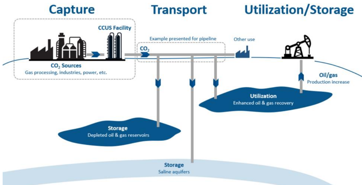
Figure 1: CCUS Schematics
