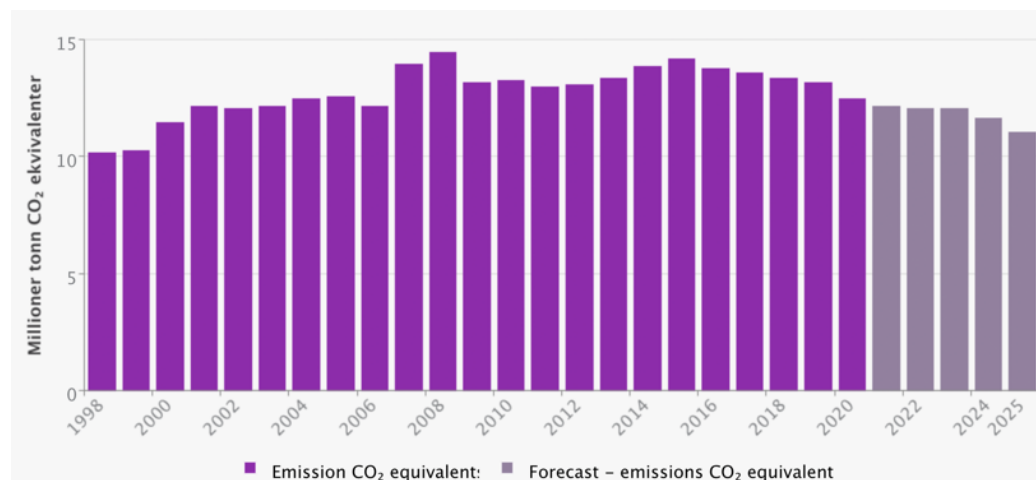
Figure 8: Emissions of Greenhouse Gases from the Norwegian Petroleum Sector
