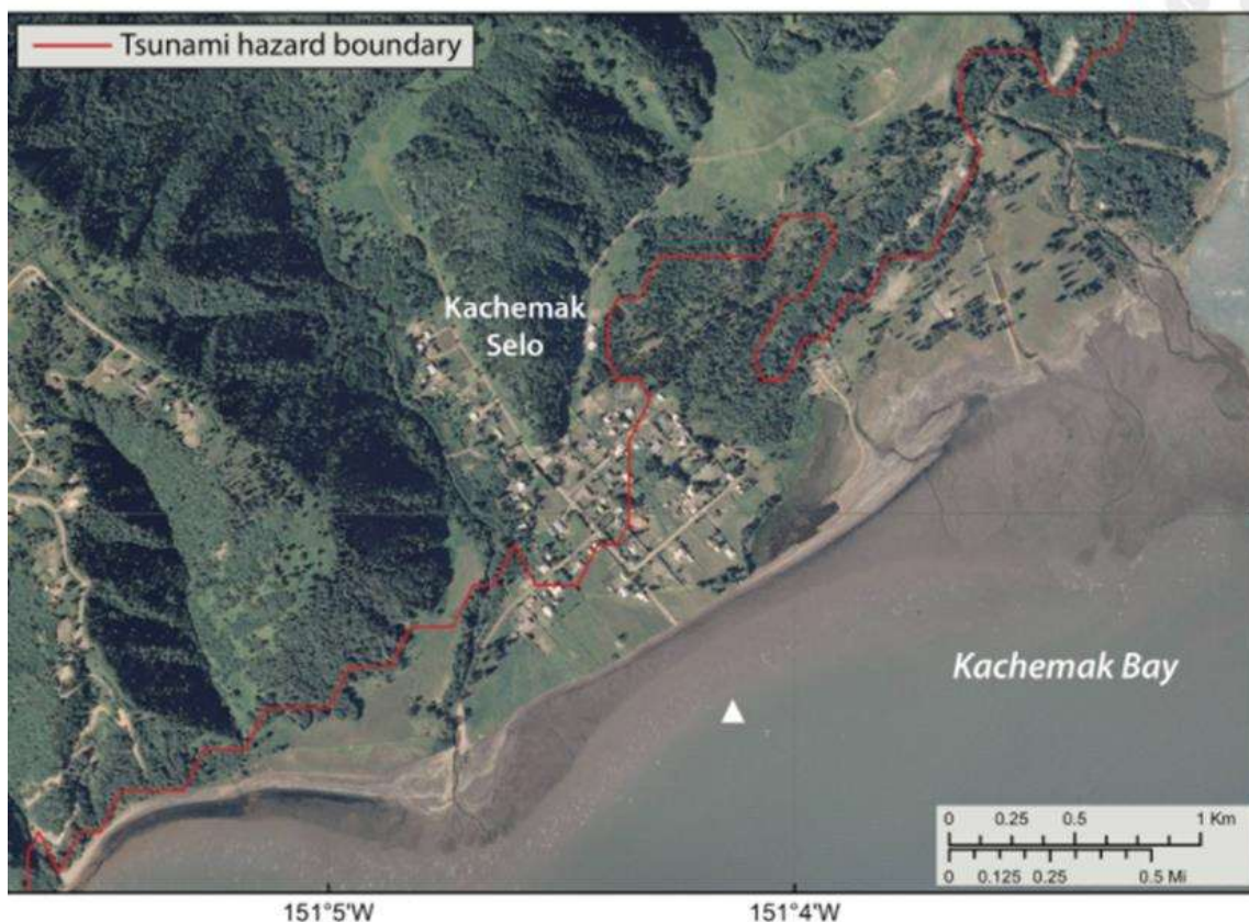
Figure 20: Tsunami Hazard Boundary in Kachemak Selo
