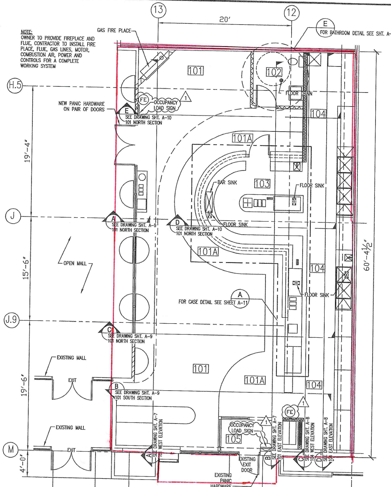
FLOOR PLAN 1/4"=1'-0" NORTH
